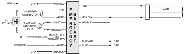
FIG 109aBH ONE (1) 36 W - 55 W LAMP WITHOUT AC BALLAST
