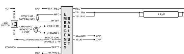
FIG 109BH ONE (1) 21 W - 54 W LAMP WITHOUT AC BALLAST
