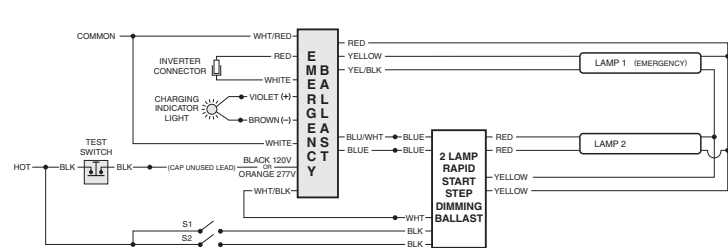
FIG 124BH TWO (2) LAMP RAPID START STEP DIMMING BALLAST
